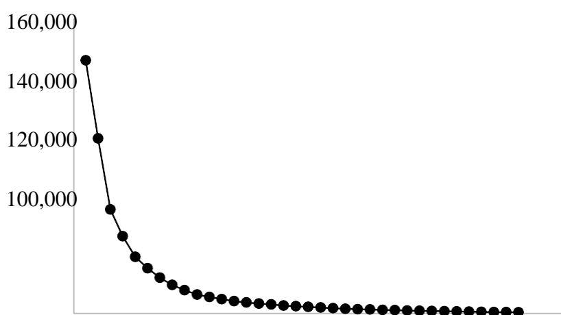
Figure 3 - Hierarchical Cluster Analysis with Furthest Neighbor Method
