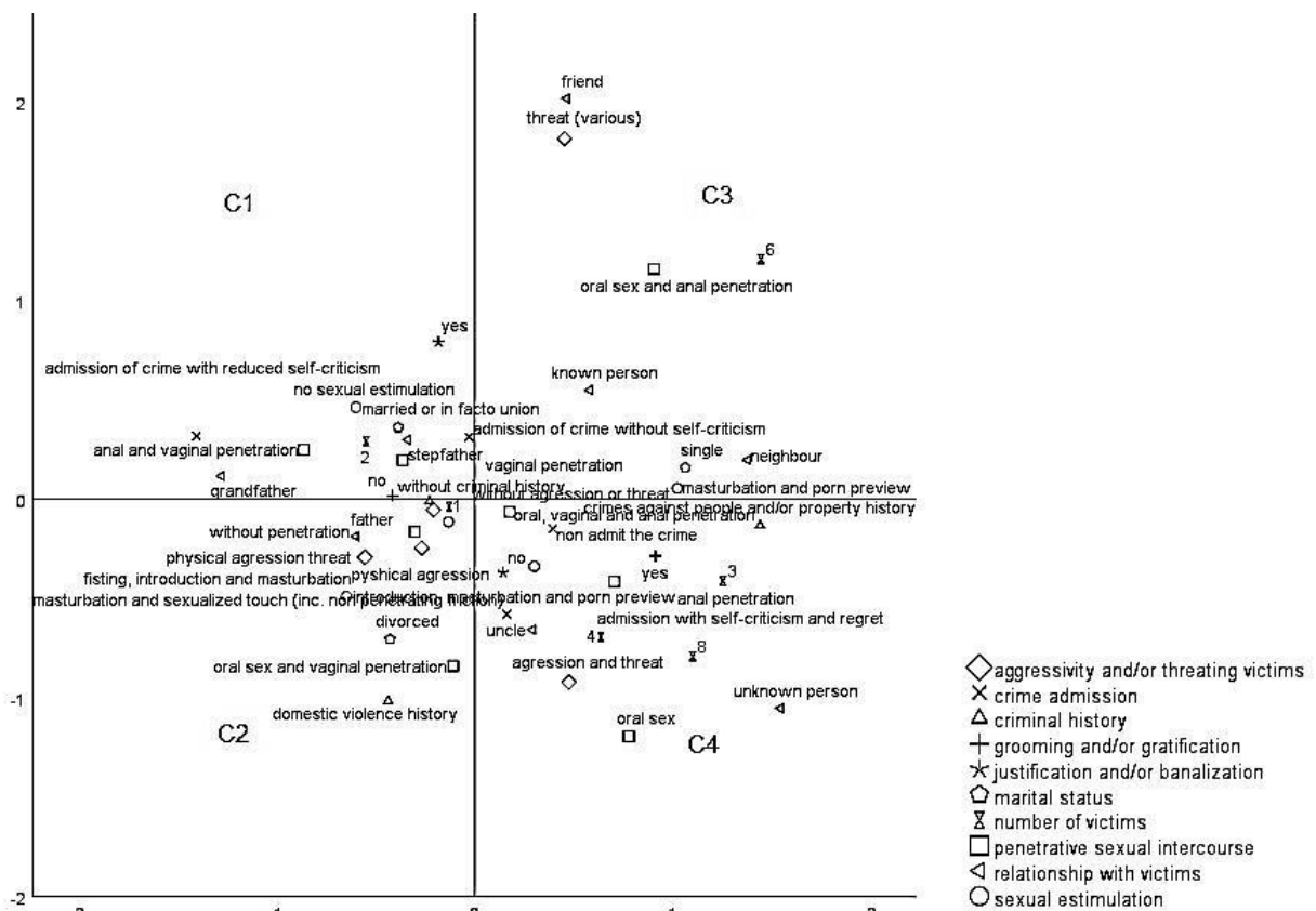
Figure 1. Multiple correspondence analysis maps with dimensional themes and
