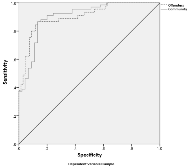
Figure 4. ROC curve
