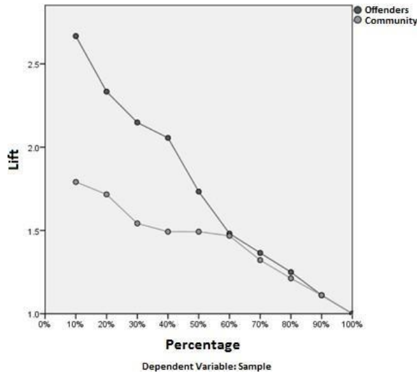
Figure 6. Lift Charts
