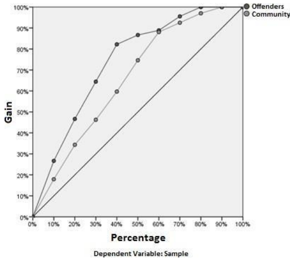
Figure 5. Cumulative Gains
