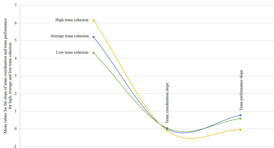
FIGURE 4 | Interteam mediation growth trajectories for the relationship between team cohesion and team performance, through team coordination, when initial team cohesion is low, medium, and high.
