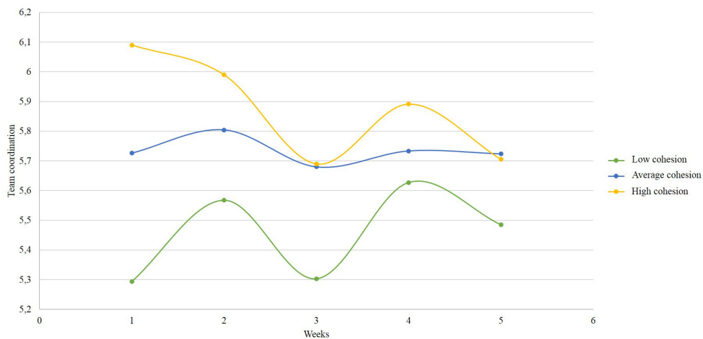
FIGURE 3 | Interteam growth trajectories for team coordination over time, when initial team cohesion is low, medium, and high.
