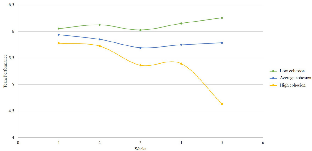
FIGURE 2 | Interteam growth trajectories for team performance over time, when initial team cohesion is low, medium, and high.
