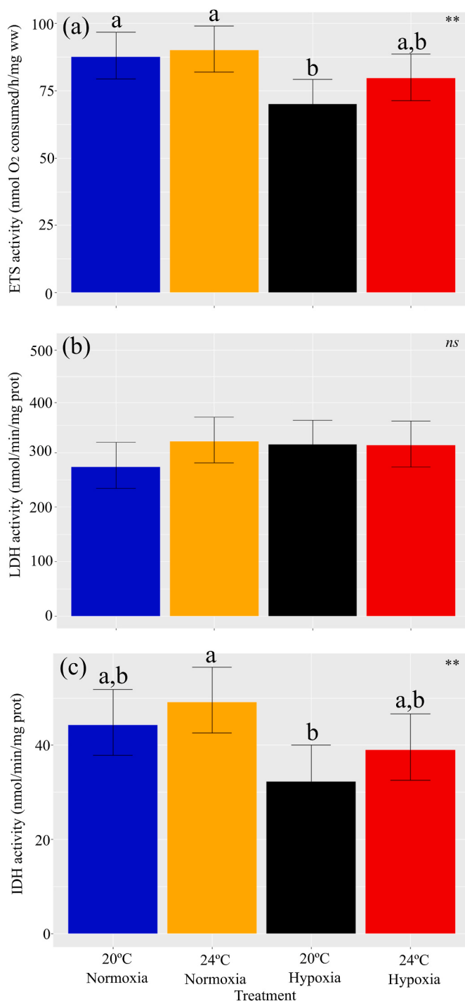
Fig. 6. Variability of biomarkers (average \pm S.E.) as responses to energy metabolism in larval tissues of seabream early stages (N = 8) chronically exposed to different treatments. ETS = Electron transport system, LDH = lactate dehydrogenase, IDH = isocitrate dehydrogenase. Letters represent homogeneous groups. ns, non-significant; ***p < 0.001; **p < 0.01; *p < 0.05.
