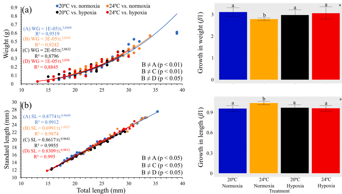
Fig. 2. Relationships between morphometric variables and the average ( \pm S.E.) of growth coefficients of seabream early stages ( N = 36 ) chronically exposed to different treatments simulating (A) control (or natural) condition, (B) warming, (C) hypoxia and (D) the combination of both stressors. Growth coefficients ( \beta_1 ) and R^2 values were calculated according to the model y = \beta_0 TL \beta_1 + \varepsilon . Letters represent homogeneous groups. ns, non-significant; *** p < 0.001 ; ** p < 0.01 ; * p < 0.05 .
