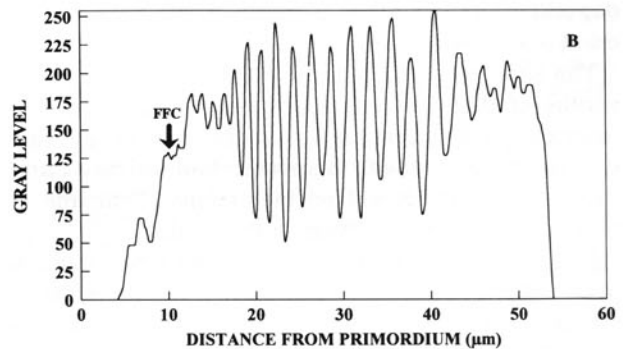
Fig. 8. Sprattus sprattus . (A) Larval otolith (processed image) (standard length of larva 15.5 mm). (B) Gray scale index at each pixel along the line indicated in (A). Discontinuous (black) and incremental (white) zones of each daily growth increment are shown (0 = black, 255 = white). FFC: first feeding check
